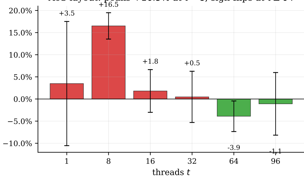
AoS layout: peaks +16.5% at t = 8 , sign-flips at t \geq 64
